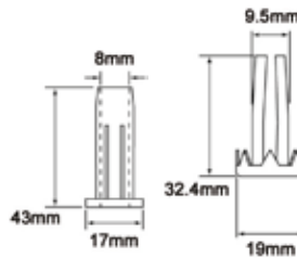
Plastic Socket
