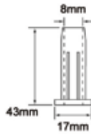
Plastic Socket
